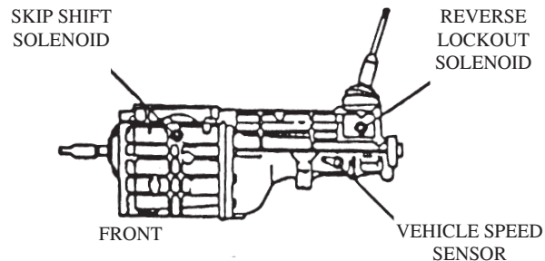
BORG-WARNER (T56) 6-SPEED MANUAL TRANSMISSION
